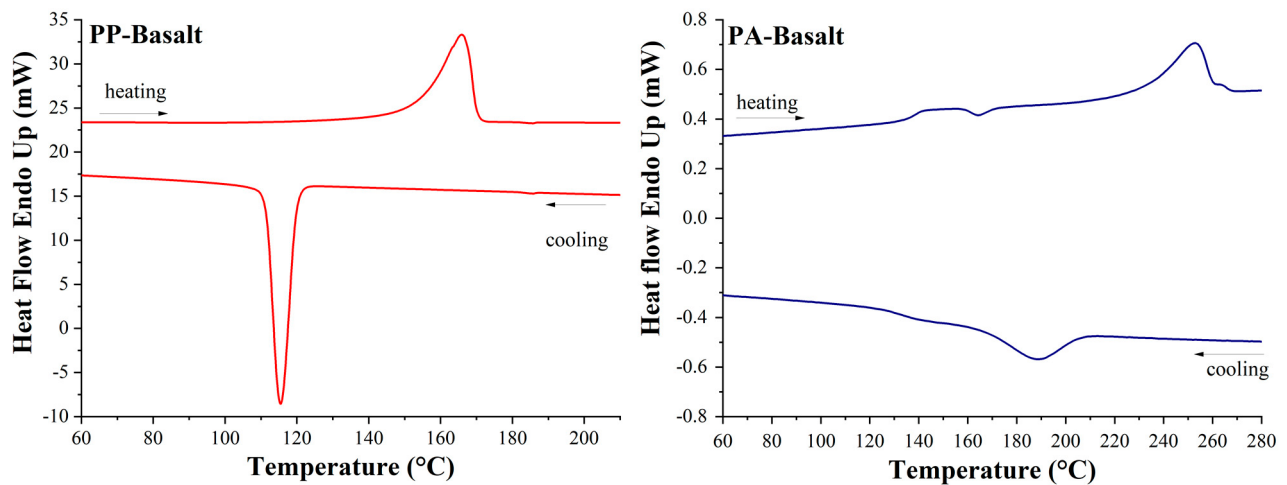
Figure 3. DSC curves of PP and PA12 basalt-filled filaments.
