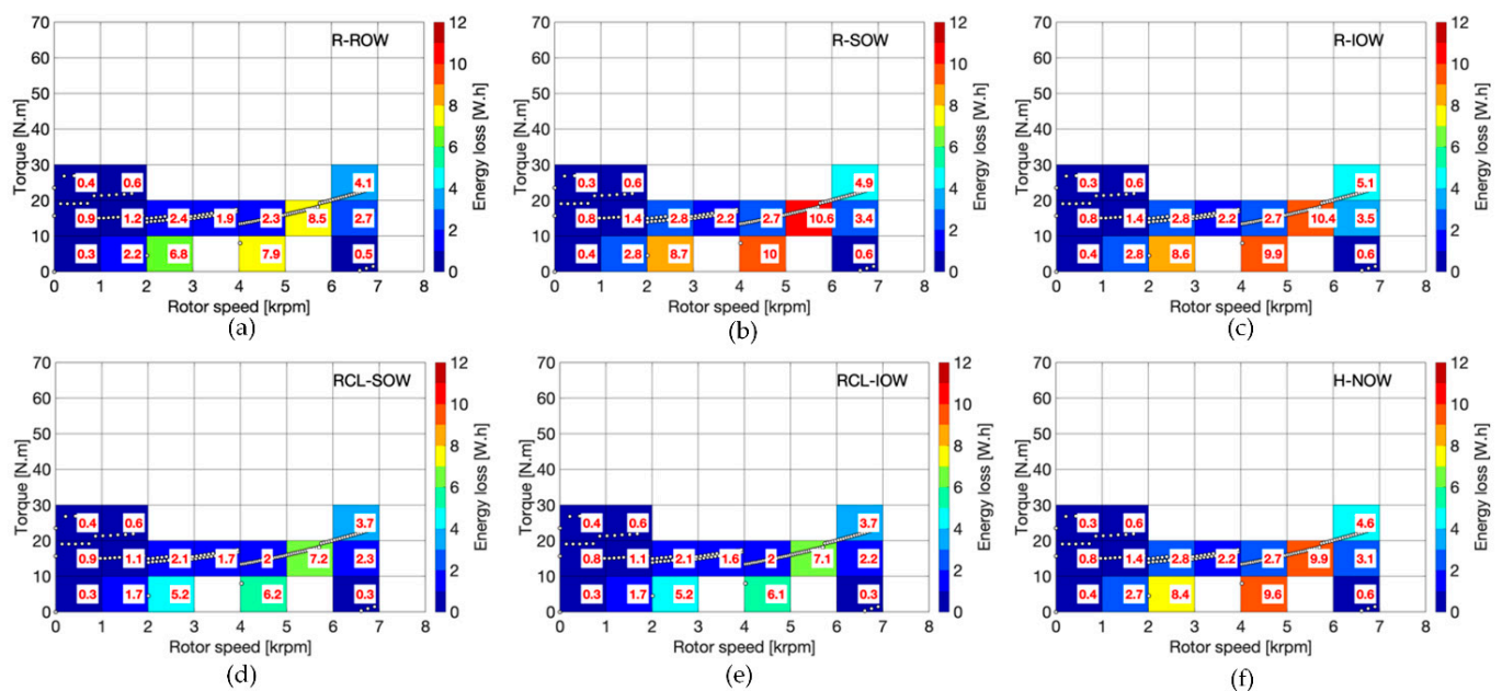
Figure 10. Energy loss distributions for the IPMSM with (a) R-ROW, (b) R-SOW, (c) R-IOW, (d) RCL-SOW, (e) RCL-IOW, and (f) H-NOW arrangements, along the NEDC driving cycle.
