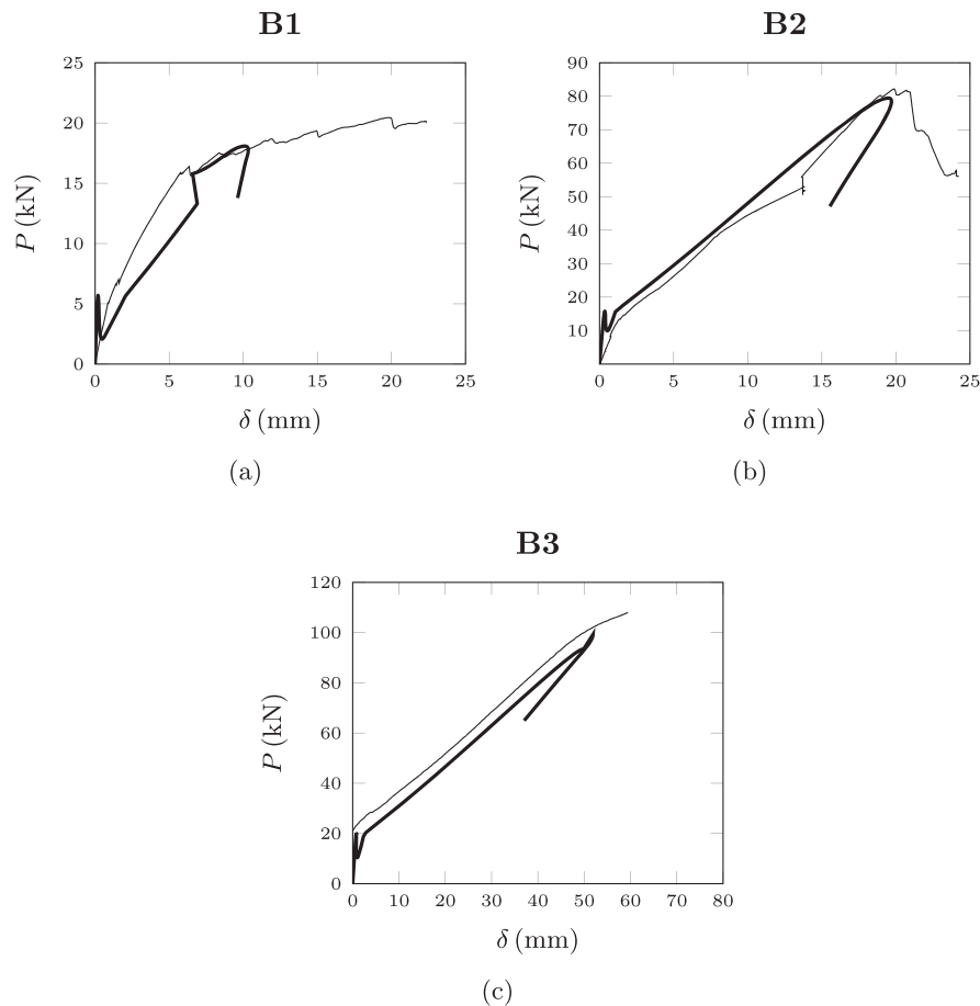
FIGURE 9 Numerical (thick) versus experimental (thin) curves: (a) h = 102 mm, (b) h = 204 mm, (c) h = 300 mm (from Toutanji and Saafi 30 ).
