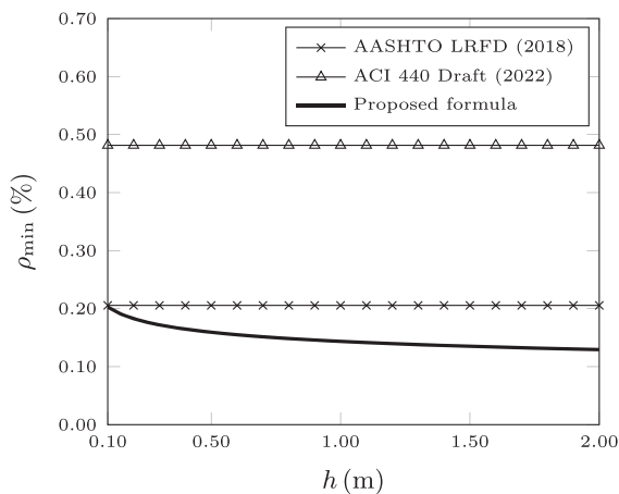
FIGURE 11 Minimum GFRP reinforcement percentage: Comparison between AASHTO 14 provisions, ACI draft, 16 and the proposed formula.
