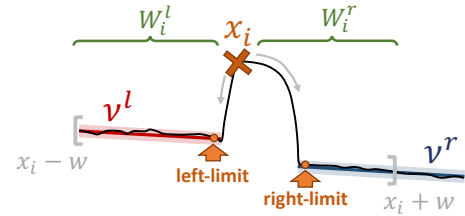
Fig. 4: Interval estimation.
