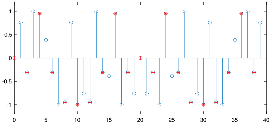
Fig. 1. The sequence \sin\left(\frac{\pi}{N} \frac{p\ell^2}{a} \left(1 + \frac{N}{a}\right)\right) for N = 20 , a = 2 , p = 1 ( \ell \in \mathbb{Z} ); cf. (1.5). Its restriction to 2\mathbb{Z} (marked in the figure above) is N -periodic.
