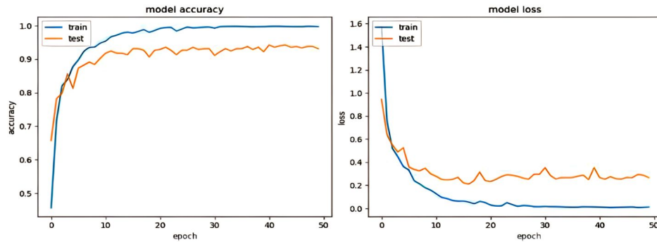
Figure 5. Graph for model accuracy and model loss
