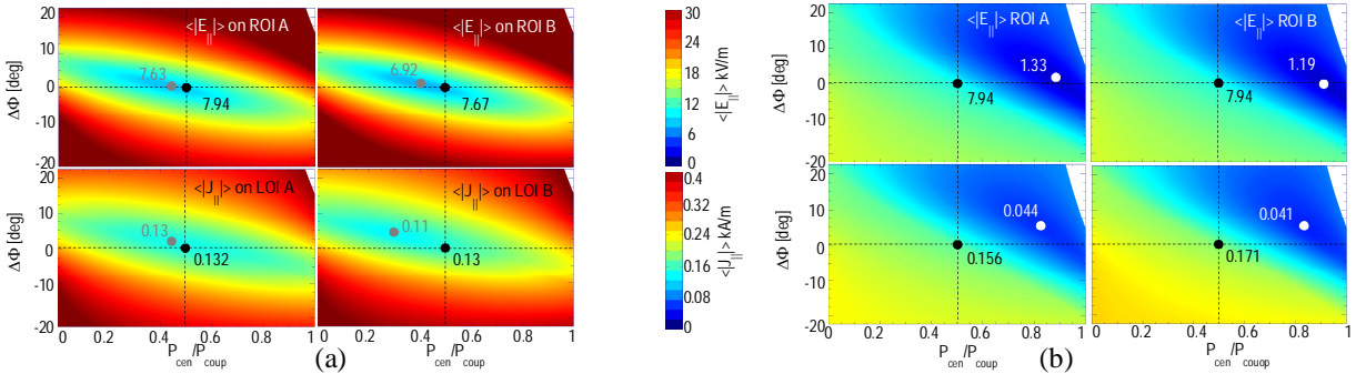
FIGURE 4. \langle E_{\parallel} \rangle on ROIs (upper row) and \langle J_{\parallel} \rangle on LOIs (lower row) as functions of P_{cen}/P_{coup} and \Delta\Phi with [0;-\pi/2] poloidal, normalized to the maximum voltage in TLs of 45 kV peak, TOPICA, 55 MHz, “large gap”: a) [0;\pi;\pi;0] ; b) [0;\pi;0;\pi] .
