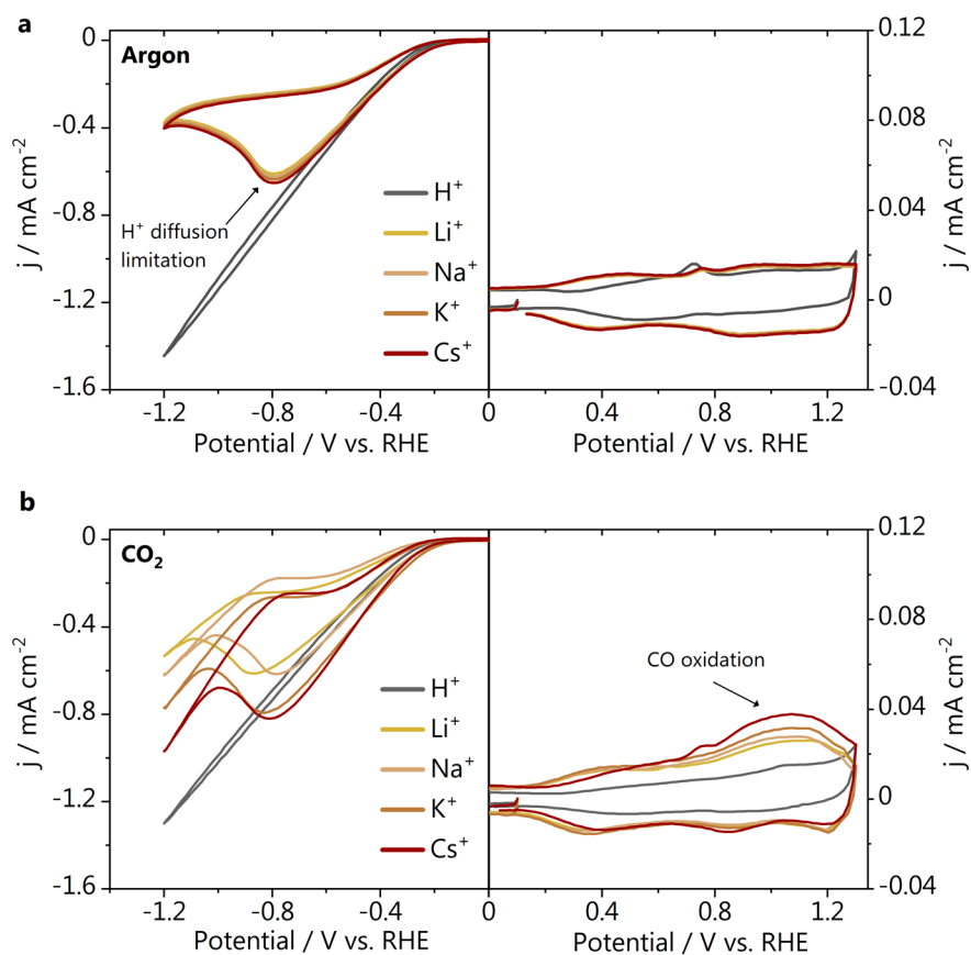
Supplementary Figure 2. Cyclic voltammetry recorded in a , argon and b , CO 2 atmosphere on gold in 1 mM M_2SO_4 ( M = H, Li, Na, K, Cs ) at pH = 3 ( 50 \text{ mV s}^{-1} ).
