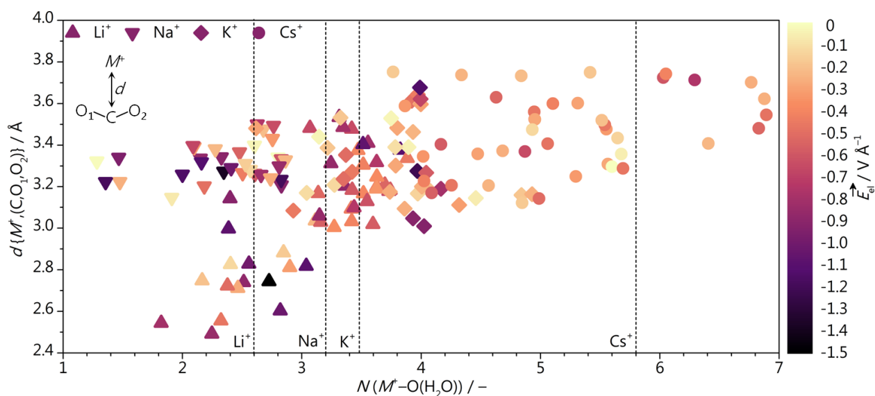
Supplementary Figure 11. Cation-induced electric field as a function of the cation-water coordination number, N(M^+-O(H_2O)) , (horizontal axis) and the average between cation-(C,O 1 ,O 2 ) distances (vertical axis) for different AIMD configurations. \blacktriangle , \blacktriangledown , \blacklozenge , and \bullet represent Li + , Na + , K + , and Cs + respectively. Dashed lines represent average cation-water coordination numbers and are taken from Supplementary Table 2.
