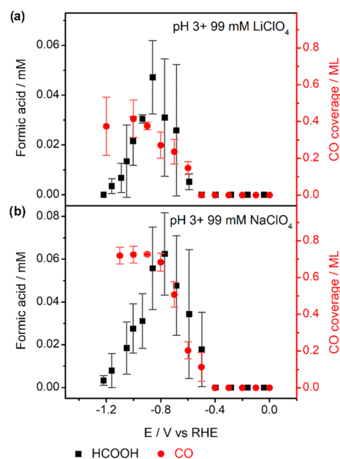
Figure 4. Cation identity effect on Pd_{ML}Pt(111) . CO coverage and HCOOH formation during CO_2RR obtained in CO_2 -saturated pH 3 electrolytes containing 99 mM (a) LiClO_4 and (b) NaClO_4 . Error bars are standard deviations based on three independent measurements.
