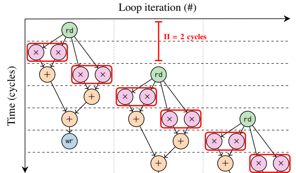
(c) Execution with II 2 cycles
