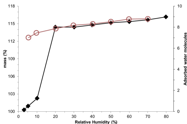
Figure 5. Water vapour isotherm starting from \gamma - 1^{c/c} . Solid symbols represent adsorption. Open symbols represent desorption. Lines are provided to guide the eye.
