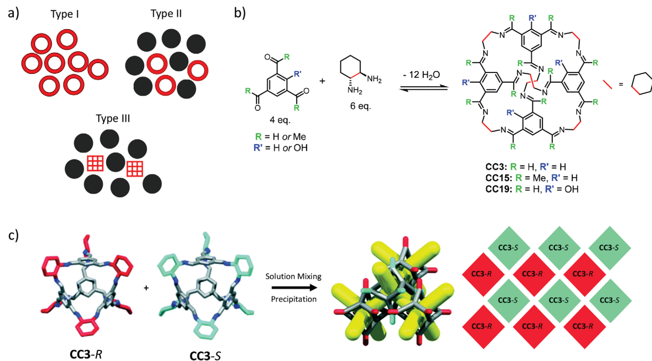
Figure 1. a) Scheme showing the three classifications of porous liquids: Type I, Type II, and Type III. b) General reaction scheme for the synthesis of CC3, CC15, and CC19, which are the POCs used to form microparticles in this study. Two cage enantiomers can be formed for each species; for example, CC3-R and CC3-S can be formed by using the different enantiomers of trans -1,2-cyclohexyldiamine (CHDA), ( R,R )-CHDA, and ( S,S )-CHDA. c) POCs such as CC3 can pack together window-to-window to form a 3D diamondoid pore network in the solid state by chiral recognition between the two cage enantiomers, which can be exploited to form POC microparticles for processing into Type III porous liquids. [19]
