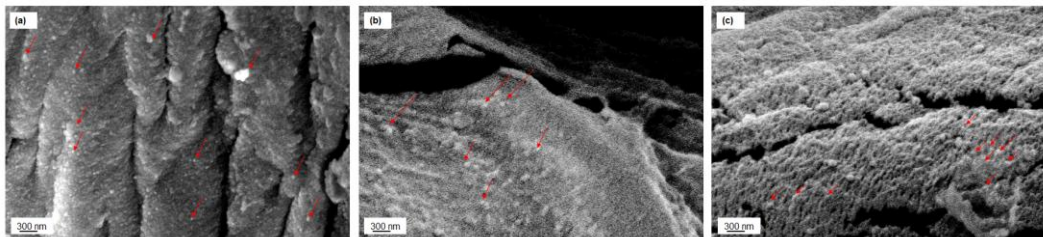
Fig. 6 FESEM images in back scattered mode of cotton with coatings, (a) SiO 2 -Ag 5 , (b) Al 2 O 3 -Ag 5 and (c) ZrO 2 -Ag 5 . The red arrows indicate the presence of Ag nanoclusters on the coating surface.
