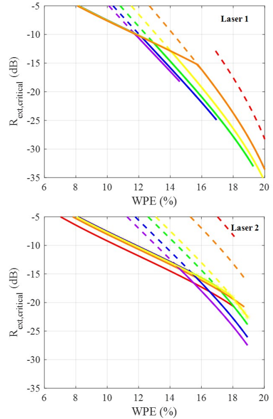
Fig. 6. Critical feedback level R_{ext,critical} as function of the WPE of Laser 1 and Laser 2 (colors are the same as in Fig.4 and Fig.5). Dashed line is the LK limit R_{ext,LK} , whereas solid line is the limit according to Eq. (11).
