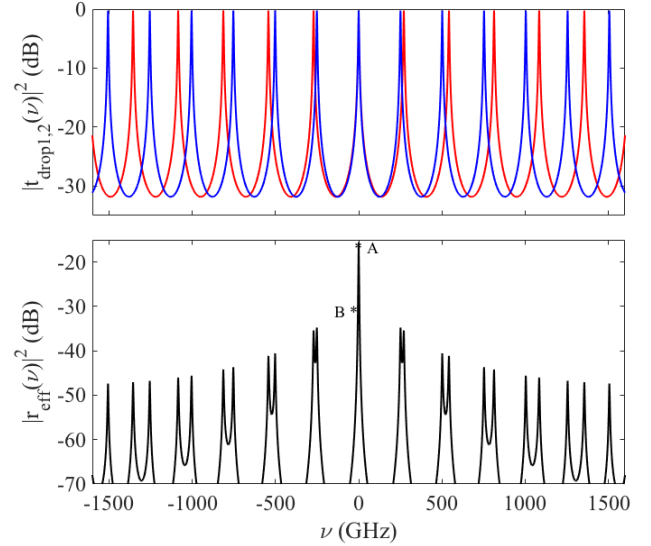
Fig. 2. Example of application of the Vernier principle of Laser 2 that provides a narrow band effective reflectivity |r_{eff}(\nu)|^2 shown in thick black line in the bottom panel. The red and blue lines in the upper panel are the drop transmission coefficients t_{drop,1} and t_{drop,2} of the two rings.
