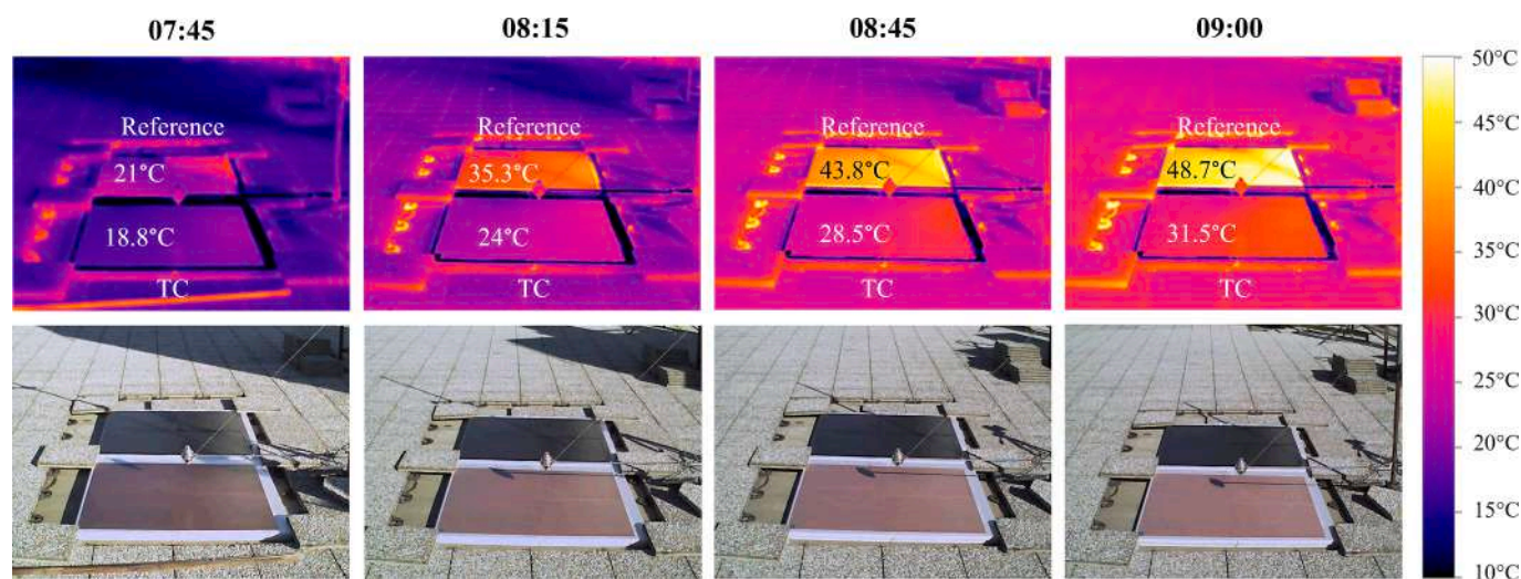
Fig. 9. Thermal images and corresponding true-color pictures of the TC/reference roof components during the switching process on the 2nd day of experimentation.
