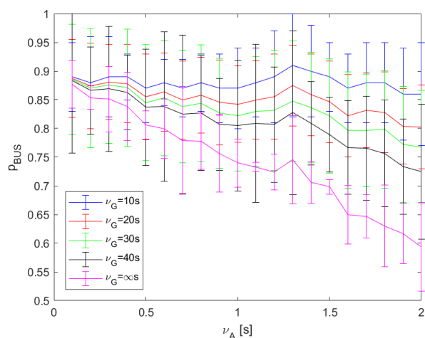
FIGURE 14. p_{BUS} of the RF for different values of \nu_A and \nu_G .
