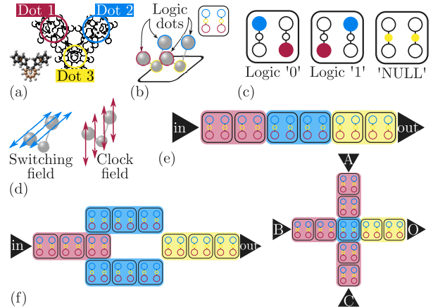
Fig. 1. Basic concepts on molFCN technology: (a) di-ferrocenyl carborane molecule geometry with a schematic view where functional dots are highlighted, (b) schematic unit cell composed of two juxtaposed molecules with the top view of the cell, (c) convention of the logic values, where full dots indicate the presence of a positive charge, (d) the direction of the switching and clock fields referred to the molecule, (e) simple wire, each background color represents a different clock region, (f) double-branch inverter and majority voter layouts for molFCN technology.
