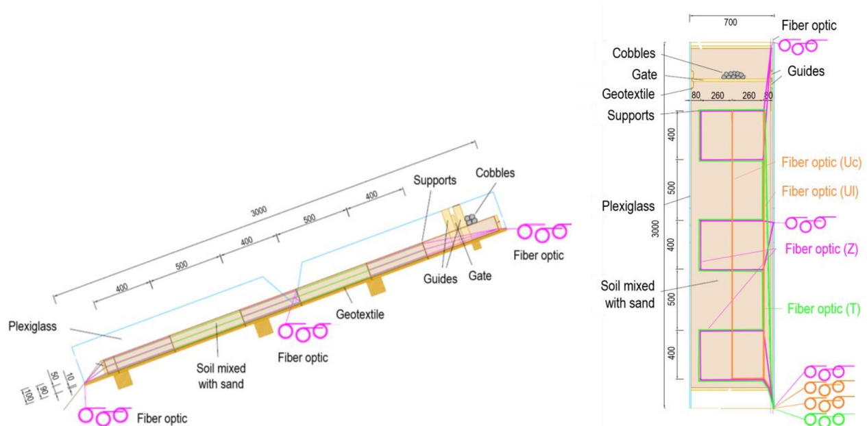
Fig. 2. Cross section and plan view of the lab-scale model with an indication of the different optical fibers installation schemes (T, U and Z).
