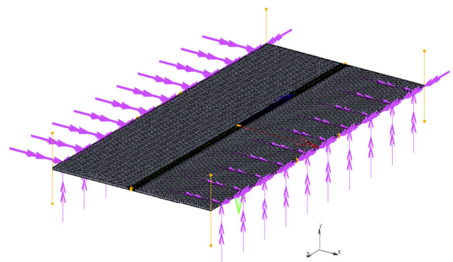
Fig. 2 Meshed model
