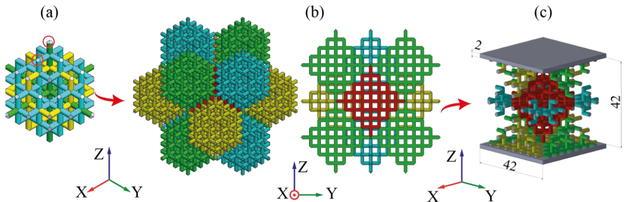
Fig. 3. (a) Chamfers adding (red circle); (b) space replication (left) and lateral-section (right); (c) cubic sample after cuts.
