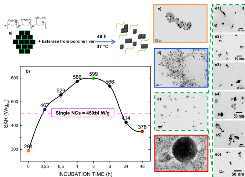
Figure 5. SAR values of 2D-MNBs exposed to esterase enzymes at different incubation times. (a) Graphical representation of the esterase-mediated cleavage of 2D-MNBs (300 \mu L, 2.2 g Fe /L), incubated at 37 °C. (b) Plot defines the variation in the SAR as a function of incubation time with esterase, measured at 300 kHz, 16 kA m -1 (which is below the biologically acceptable limit H_f = 5 \times 10^9 A m -1 s -1 ). The horizontal dashed line corresponds to the SAR value of single IONCs (450 \pm 4 W/g). The TEM images on the right panel indicate the structural morphology of cleaved 2D-MNBs at different time points of incubation, including (c) 0 h (before the addition of enzyme, highlighted in orange), (d) 0.25 h (blue), (e) 3 h (green), and (f) 48 h (red). Additional images framed in green (e1–e6), correspond to the sample at 3 h. At this time point, small chains of NCs appeared, which may explain how the highest SAR recorded was achieved, owing to their unique structural arrangements.
