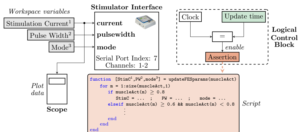
Figure 7. Simulink® model for the online control of the RehaStim 2 FES stimulator. The stimulation parameters are updated by running a MATLAB® script every (Update time).
