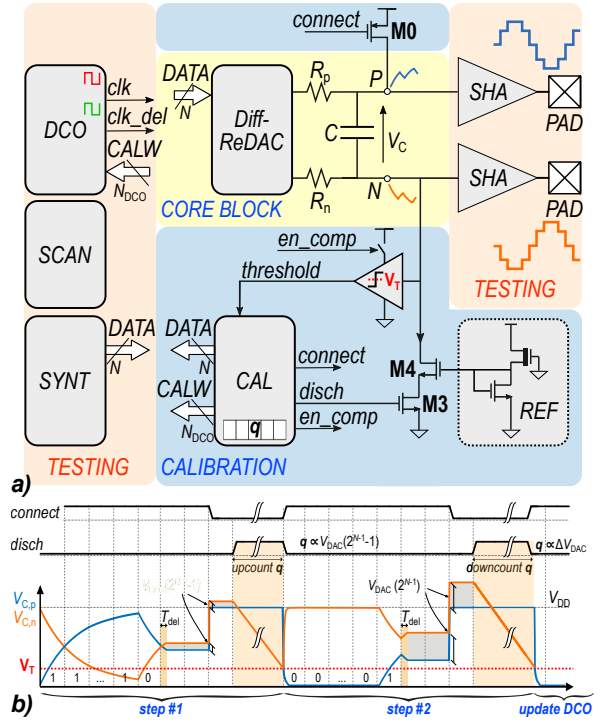
Fig. 3. Chip-level architecture (a), CAL timing diagram (b).
