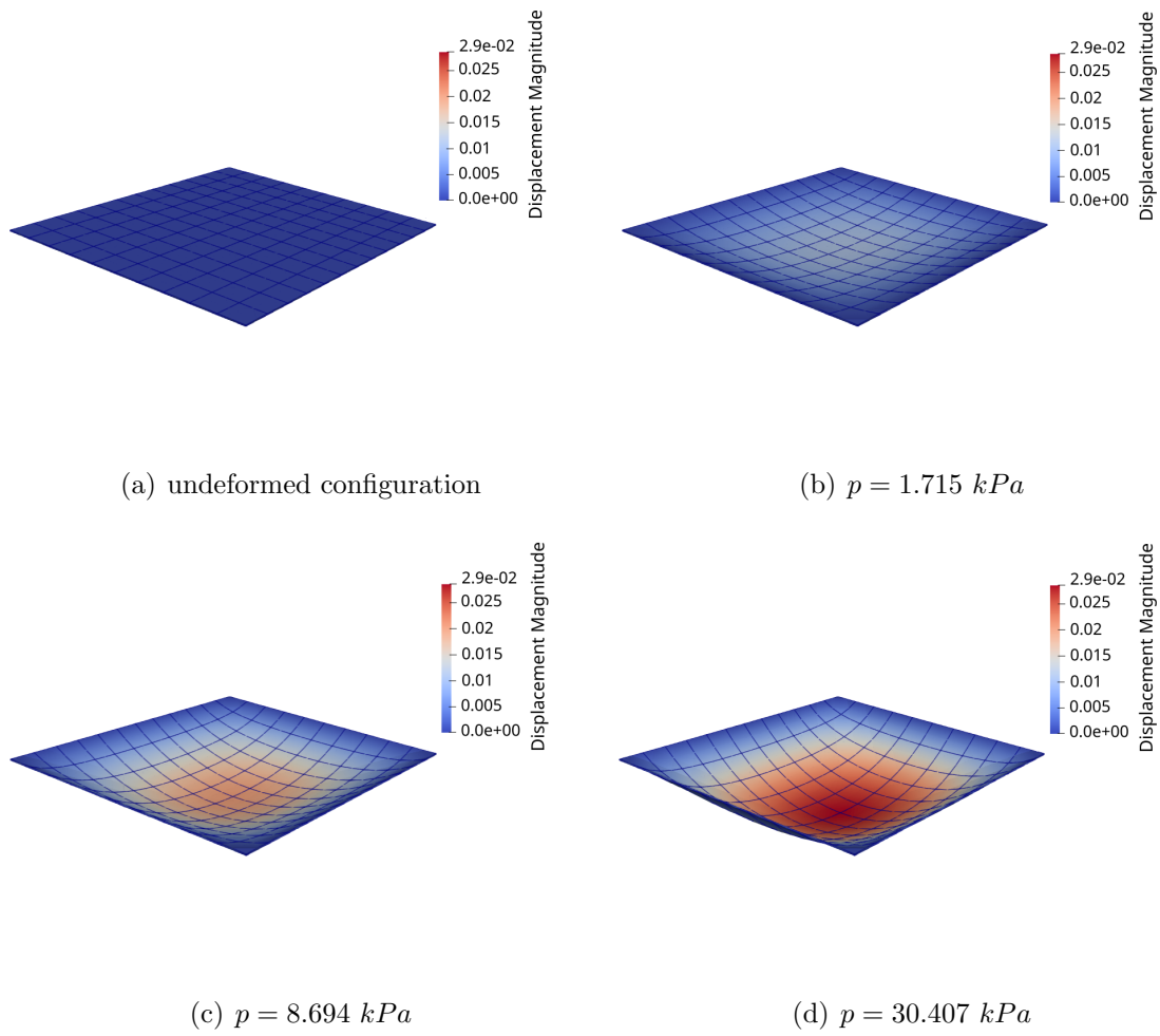
Figure 9: Undeformed and deformed states of the simply supported rectangular plate. 12 \times 10 Q9 model.
