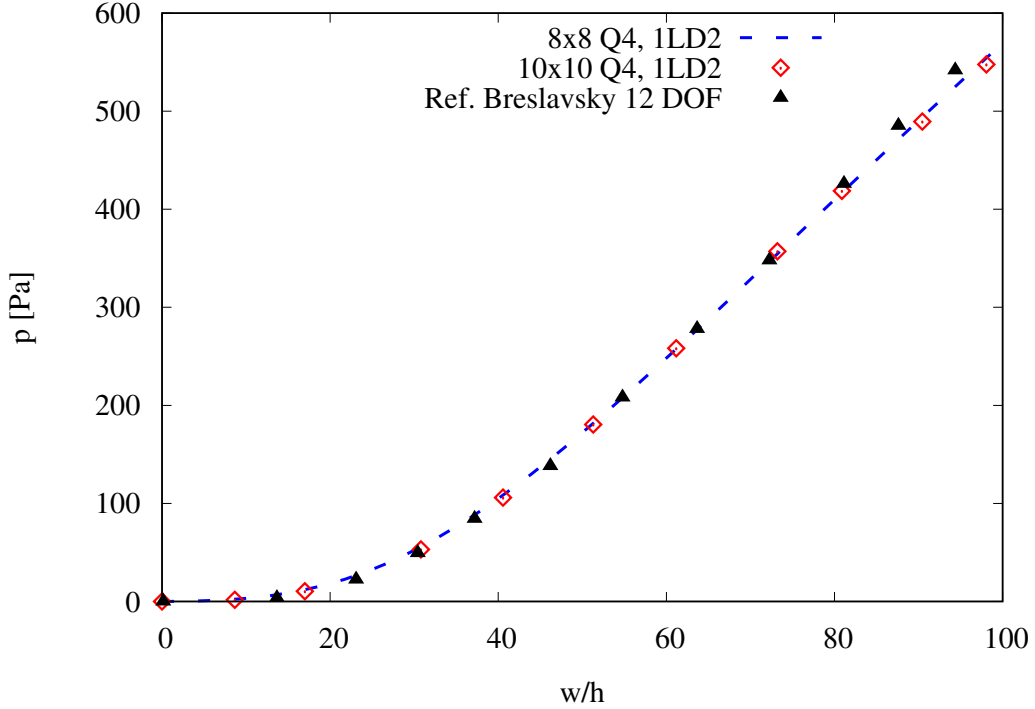
Figure 5: Pressure load-midpoint deflection response of the biological material plate. Comparison between two different numbers of element and solution with 12 DOF of Breslavsky [19].
