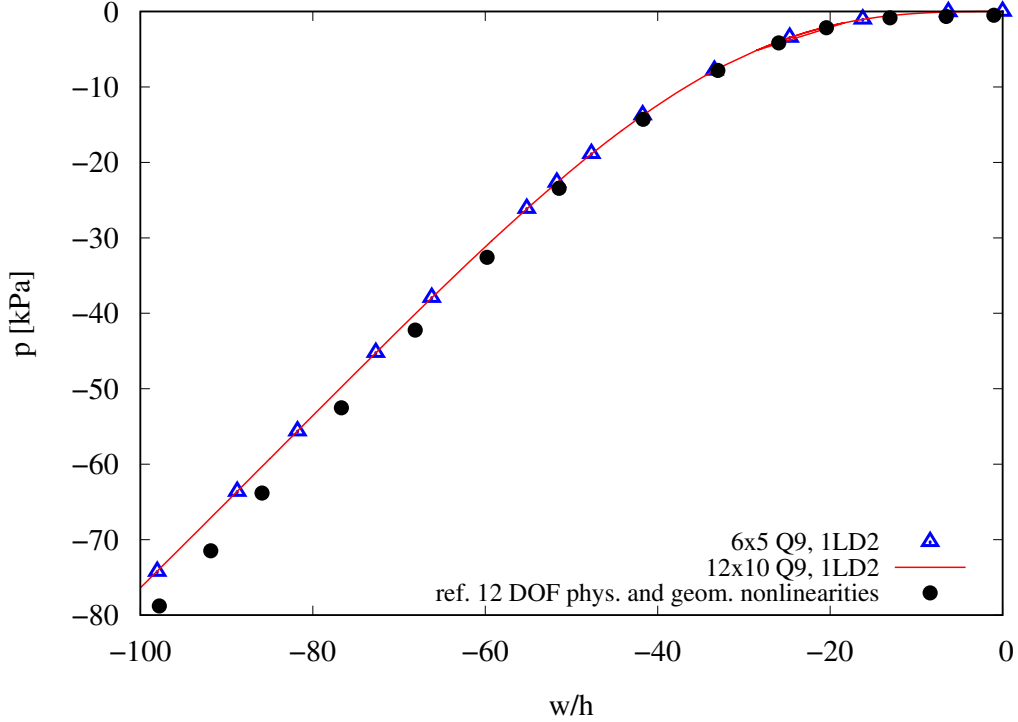
Figure 7: Middle point deflection-pressure curves for models with geometrical and physical nonlinearity . Comparison between 6 \times 5 Q9, 12 \times 10 Q9 and solution with 12 DOF of Breslavsky [18].
