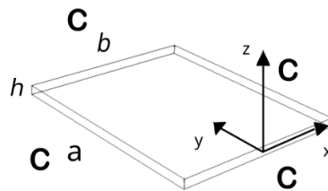
Figure 10: Boundary condition and geometry of the silicone rubber plate.
