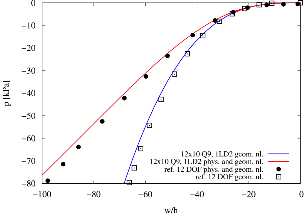
Figure 8: Middle point deflection-pressure curves for 12 \times 10 Q9 model and \nu = 0.4999 . Comparison between solution with geometrical nonlinearities only and solution with both geometrical and physical nonlinearities. Comparison with 12 DOF Breslavsky's solution [18].
