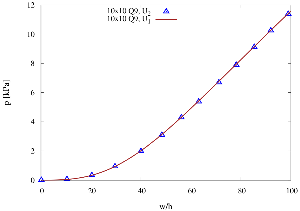
Figure 4: Neo-Hookean plate pressure–deflection response. Deflection measured at the centre of the thin plate considering two different volumetric function U_1 and U_2 .
