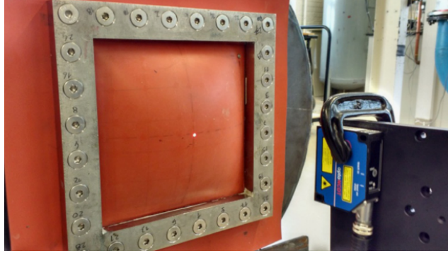
Figure 11: Silicone rubber plate under a pressure of 1 Psi. The deflection at the centre point is measured using a Micro-Epsilon triangulation laser sensor [20]. Adapted from [20] with permission from Elsevier.
