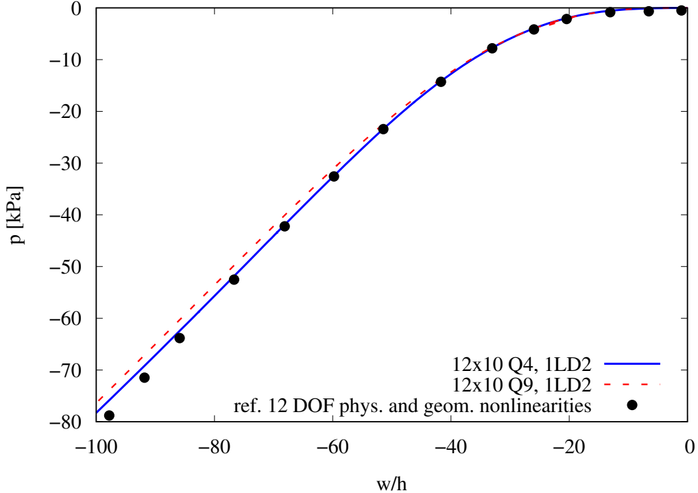
Figure 6: Middle point deflection-pressure curves for models with geometrical and physical nonlinearities . Comparison between two different models 12 \times 10 Q4, 12 \times 10 Q9 and solution with 12 DOF of Breslavsky [18].
