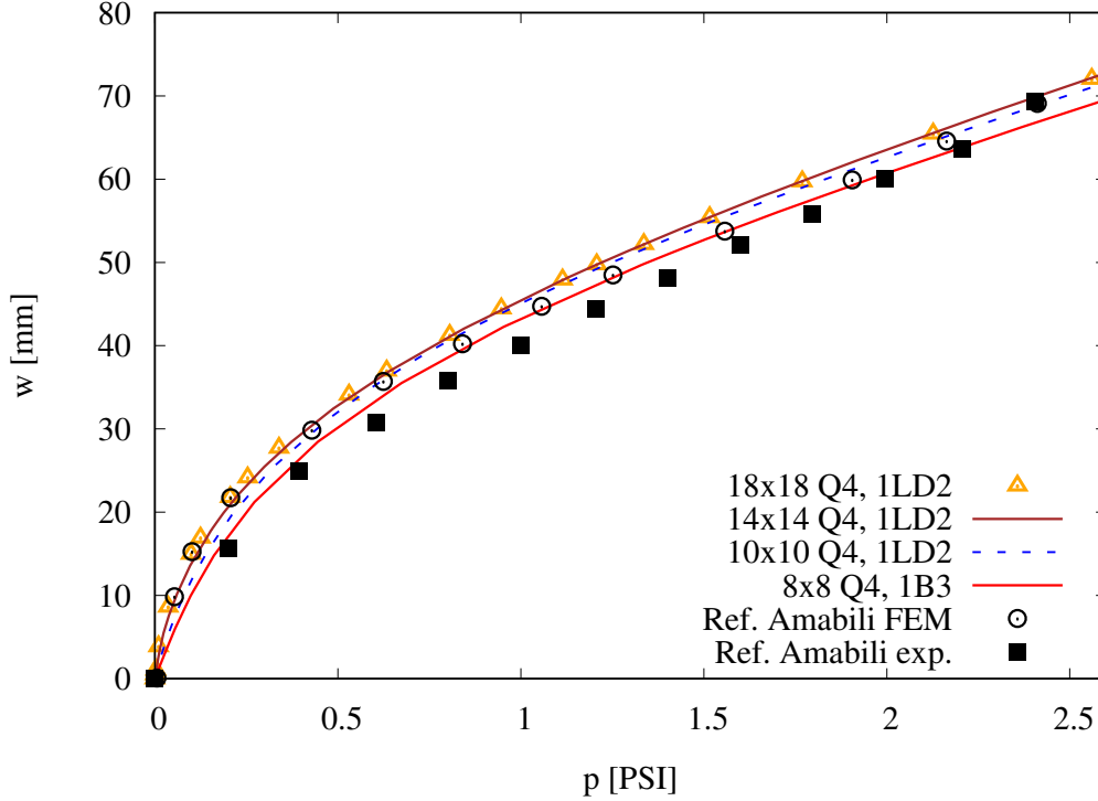
Figure 12: Static deflection of the silicone plate measured at the centre as function of the pressure. Comparison between different FEM models and experimental and FEM solutions of Amabili et al [20] .
