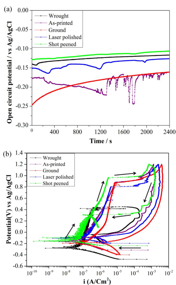
Fig. 10 – (a) Open circuit potential measurements, (b) Cyclic potentiodynamic polarization curves for all samples in 0.9% NaCl.
