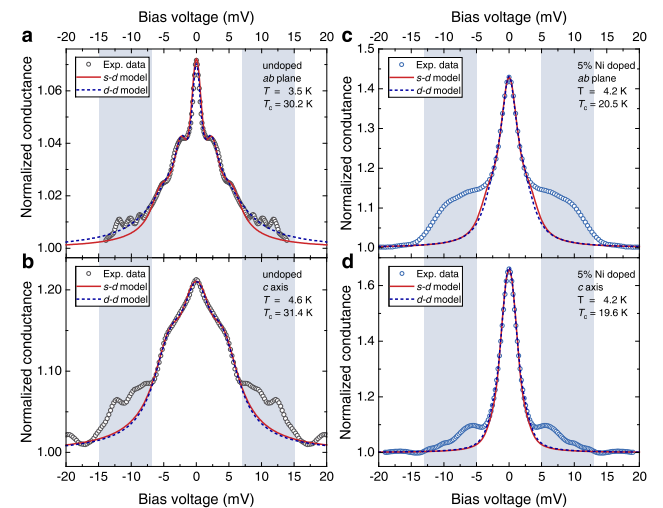
Fig. 9. (Color online) Low-temperature directional PCARS spectra (symbols) on single crystals of \text{RbCa}_2(\text{Fe}_{1-x}\text{Ni}_x)_4\text{As}_4\text{F}_2 with x=0 (a), (b) and x=0.05 (c), (d), and corresponding two-gap fits of the spectra either in an s-d model (solid red lines) or in a d-d model (dashed blue lines). All fitting parameters are summarized in Table 1. Adapted from Ref. 41.
