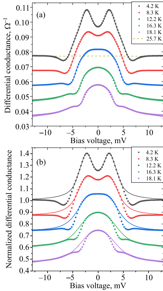
Fig. 3. (a) (Color online) As-measured, unnormalized differential conductance dI/dV of a soft point contact on Mg_{0.75}Al_{0.25}B_2 single crystal, at different temperatures (symbols) together with the relevant fits (solid lines) that include both Andreev reflection and the current-dependent Maxwell term. The dashed horizontal line is the normal-state conductance at T = 25.7 K. All the curves have been vertically offset for clarity, apart from the lowest-temperature one (black symbol) and the normal-state one. (b) Experimental point-contact curves, normalized to the actual normal-state conductance at T = 25.7 K, vertically offset for clarity and fitted to the standard 2D BTK model.
