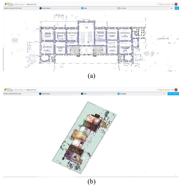
Figure 8. Point cloud alignment inside Holobuilder. Two points picking on the plan (a) and elevation definition between the point cloud and floor level (b)
