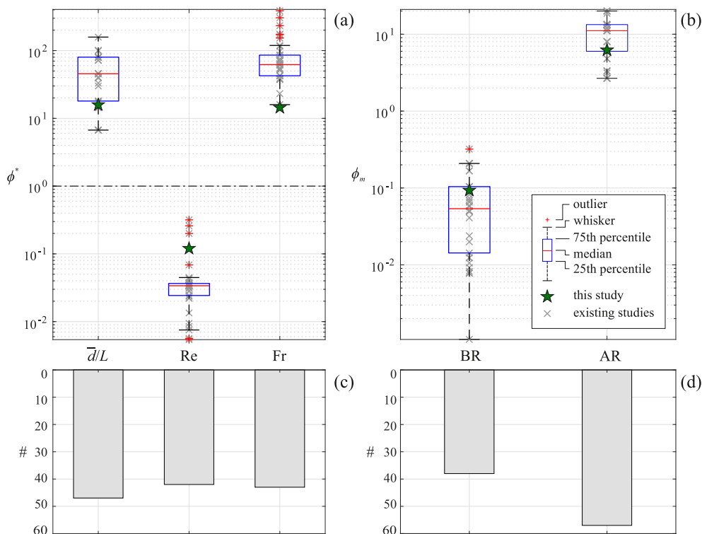
Fig. 7. Setup dimensionless numbers: similarity dimensionless numbers (geometry, Reynolds and Froude) normalized to prototype conditions (a), model blockage ratio BR and aspect ratio AR (b) and corresponding cardinality # of examined studies (c,d).
