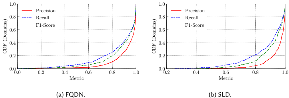
Fig. 2. F1-Score, precision and recall distributions for threat A, separately for the FQDN and second-level domain scenarios.
