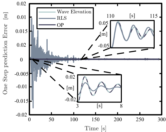
Fig. 4. One-step prediction error evolution over time: RLS and OP algorithm comparison.
