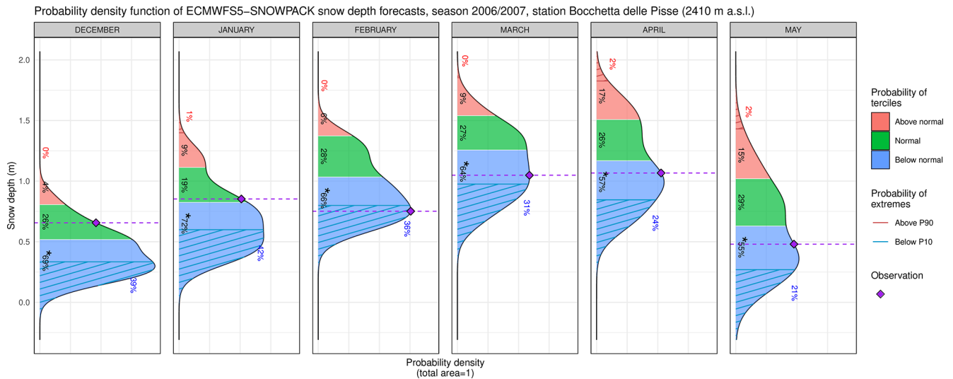
Figure 4. Probability density functions (PDFs) of the ECMWF5-SNOWPACK monthly mean snow depth ensemble forecasts for the season 2006–2007 (starting date: 1 November 2006; lead times: 2, 3, 4, 5, 6, and 7 months) and for the station of Bocchetta delle Pisse, 2410 m a.s.l. in the Italian Alps. Areas in blue, green, and coral colours represent the % probability to have monthly average snow depth below, near and above the normal conditions for the period, respectively, and the asterisk indicates the most likely tercile. Areas with blue and red parallel lines represent the probability to have monthly snow depth below the 10th percentile and above the 90th percentile, respectively. Observations are reported as purple diamonds.
