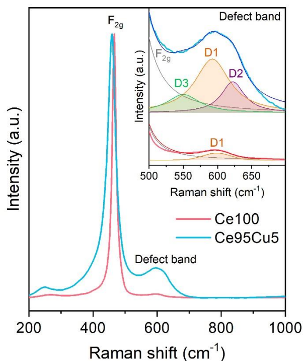
Fig. 4. Raman spectra of the two catalysts collected at RT, normalized to the F_{2g} peak intensity. In the inset, the defect band is magnified, highlighting the different deconvoluted peaks (thin lines).
