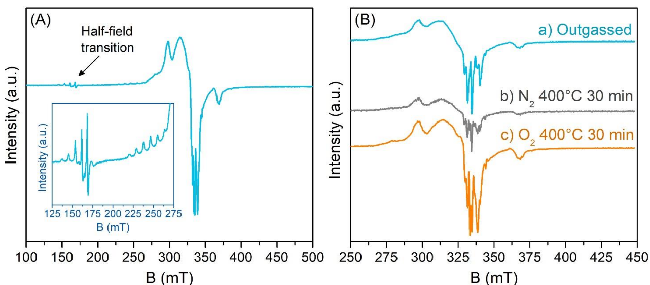
Fig. 2. Complete EPR spectrum of the Ce 95 Cu 5 sample acquired at 77 K after outgassing the powder (A); in the inset, the half-field transition region is magnified. EPR spectra collected at 77 K after treating the Ce 95 Cu 5 catalyst in different ways (B): after outgassing the sample (a), after thermal treatment in N 2 at 400 °C for 30 min (b), and after thermal treatment in O 2 at 400 °C for 30 min (c).
