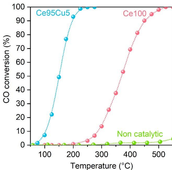
Fig. 6. Light-off curves reporting the percentage of CO converted as a function of the temperature during CO oxidation tests (feed gas mixture containing 1000 ppm of CO and 10% of O 2 in N 2 , temperature increased step by step). Results are similar to those of analogous hydrothermally-synthesized samples described in [29].
