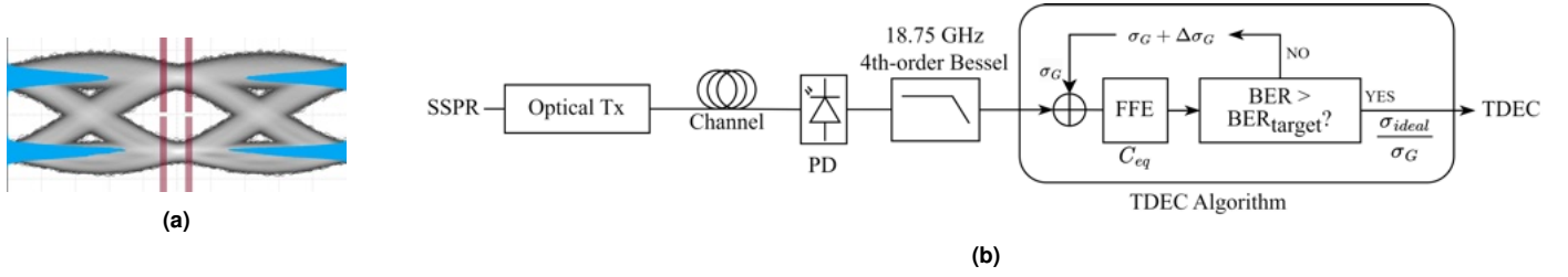
Fig. 1. (a) Eye diagram showing the four sampling windows and the resulting histograms. (b) Block diagram summarizing the TDEC evaluation procedure.
