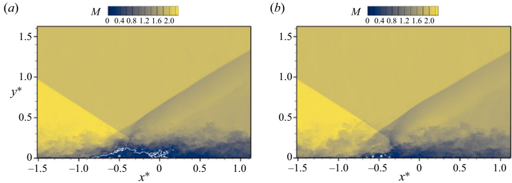
Figure 10. Instantaneous contours of the Mach number on a vertical slice for two different states during the intermittent event around t U_\infty / \delta_0 \approx 1160 . The white line indicates the points with null streamwise velocity. (a) t U_\infty / \delta_0 = 1158.1 , the area occupied by the bubble is large; (b) t U_\infty / \delta_0 = 1195.6 , the bubble is almost absent.
