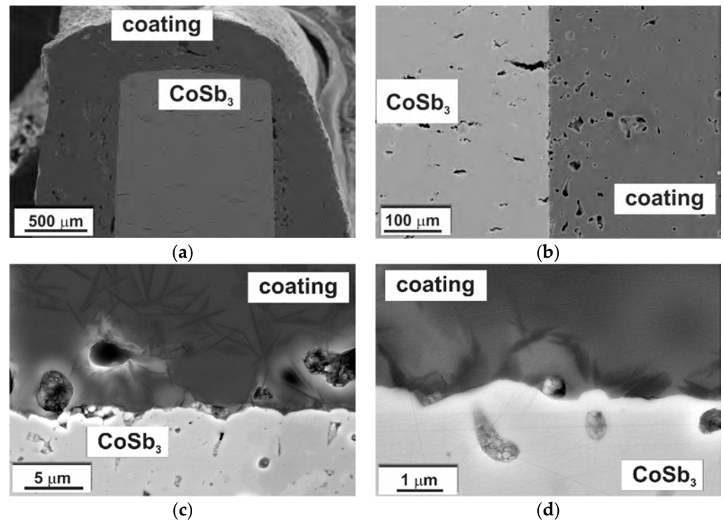
Figure 10. (a) Cross-section of the coated sample; (b–d) magnification of the interface (SEM-SE).
