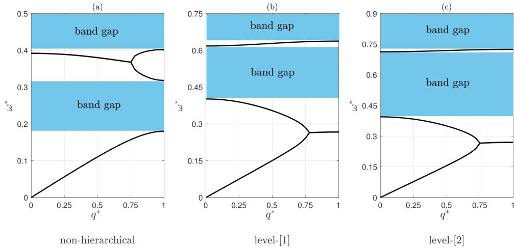
Figure 5: Non-dissipative linear elastic medium: dispersion diagrams for triangular sutures in the case of a (a) non-hierarchical and (b, c) hierarchical configuration with one (b) and two (c) levels of hierarchy. Focus on the first bandgap.
