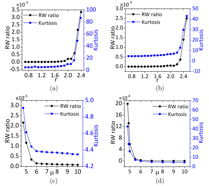
FIG. 5. Kurtosis and rogue wave ratio for (a) below \mu = 5.0 and (b) above \mu = 5.35 laser threshold with varying r . The same two parameters for varying \mu and fixed r at (c) unity and (d) r = 2.2 .
