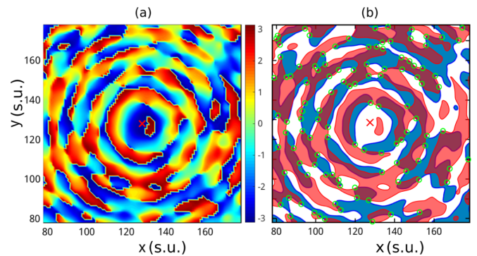
FIG. 7. (a) Phase and (b) contour plot for the real [blue (dark gray)] and imaginary [red (light gray)] parts of the electric field at the time of extreme-event occurrence in the spot highlighted by the red cross. In (b) the color-filled areas correspond to positive values for the respective variables; hence, the border of each area identifies a zero isoline. The crossings between blue and red isolines, highlighted by green circles, identify optical vortices.
