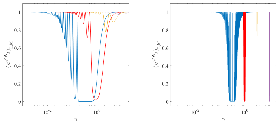
Figure 2. Values of \langle e^{-\beta W_J} \rangle_{L,M} for the single harmonic oscillator with \lambda = \sin \gamma t , as a function of the forcing frequency \gamma , for different values of \Gamma_0 volumes and different final times \tau . Left and right panels refer to L = M = 1 and L = M = 10 , respectively, with \tau such that B = \sin(2\pi) for the first case and B = \sin(200\pi) for the second. Blue, red, yellow, and purple plots refer to stiffnesses k_s = 0.1, 1, 10, 100 , respectively. Other parameters are set to m = 1, \beta = 1 , and k_D = 1 .
