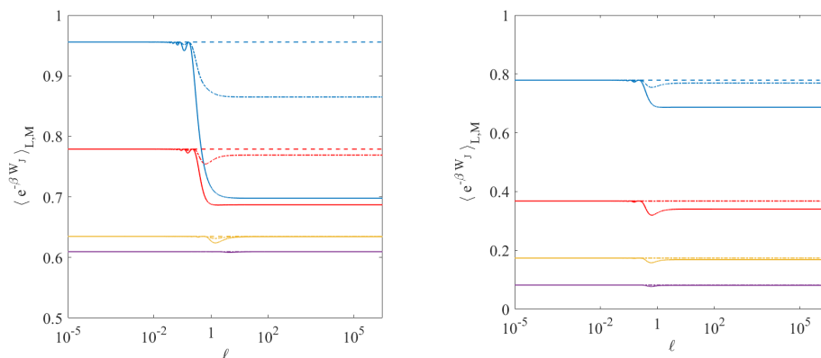
Figure 3. Values of \langle e^{-\beta W_f} \rangle_{L,M} for the single harmonic oscillator driven by a constant speed moving harmonic trap, with a final protocol value of \lambda(\tau) = B = 1 . The result is shown as a function of \ell , for different values of L and M . Solid lines refer to L = M = 1 , dash-dotted lines to L = M = 2 , and dashed lines to L = M = 5 . In the left panel, blue, red, yellow, and purple plots refer to k_p = 0.1, 1, 10, 100 , respectively. In the right panel, blue, red, yellow, and purple plots refer to \beta = 1, 4, 7, 10 , respectively. Other parameters are set to m = 1 and k_D = 1 .
