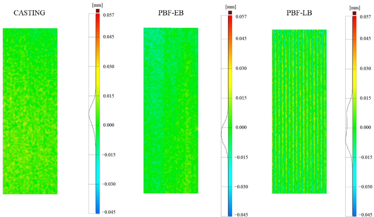
Figure 4. Surface topography images for samples produced with casting, PBF-EB, and PBF-LB, machined with the same process parameters ( t_{on} = 10 s, DC = 8.33%, I = 3 A, workpiece thickness = 20 mm).
