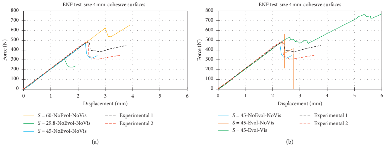
FIGURE 21: ENF test: cohesive surface approach (element size 4 mm).
