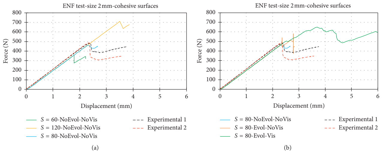
FIGURE 23: ENF test: cohesive surface approach (element size 2 mm).
