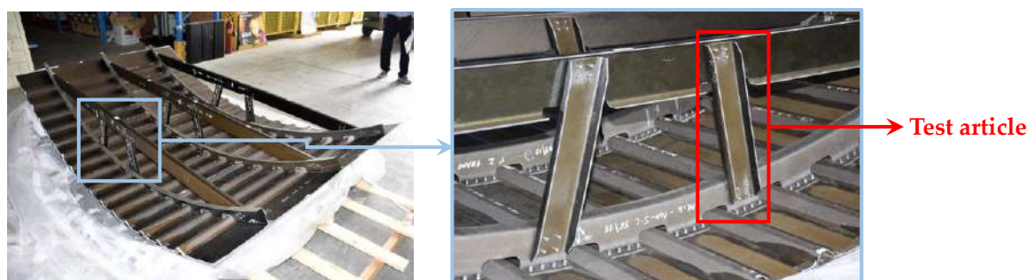
Figure 1. Location of the stanchion in a typical fuselage section.
