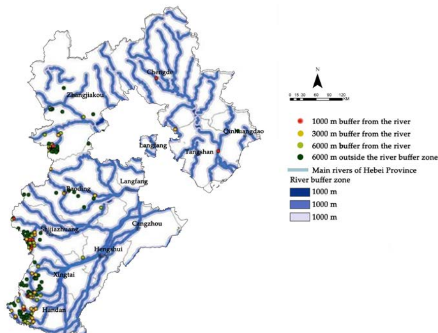
Figure 10. River Distribution of traditional villages in Hebei Province. Data source: https://www.gscloud.cn/ (accessed on 5 April 2023).
