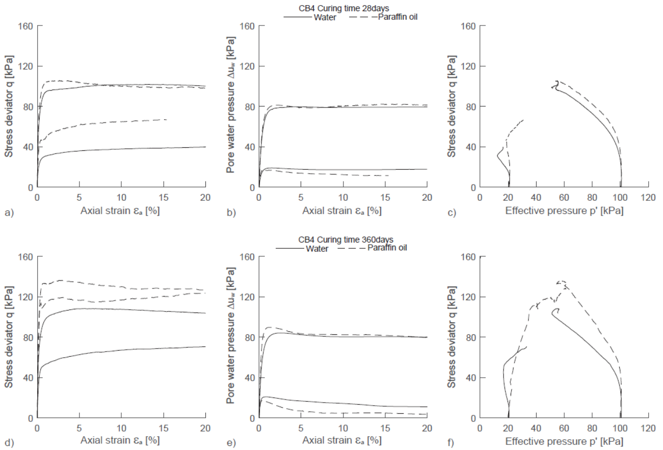
Figure 10: Mixture CB4 triaxial tests ( p'_c = 20 and 100 kPa) results: a) q - \epsilon_a plane curing 28 days, b) \Delta u_w - \epsilon_a plane curing 28 days, c) q - p' plane curing 28 days, d) q - \epsilon_a plane curing 360 days, e) \Delta u_w - \epsilon_a plane curing 360 days and f) q - p' plane curing 360 days
