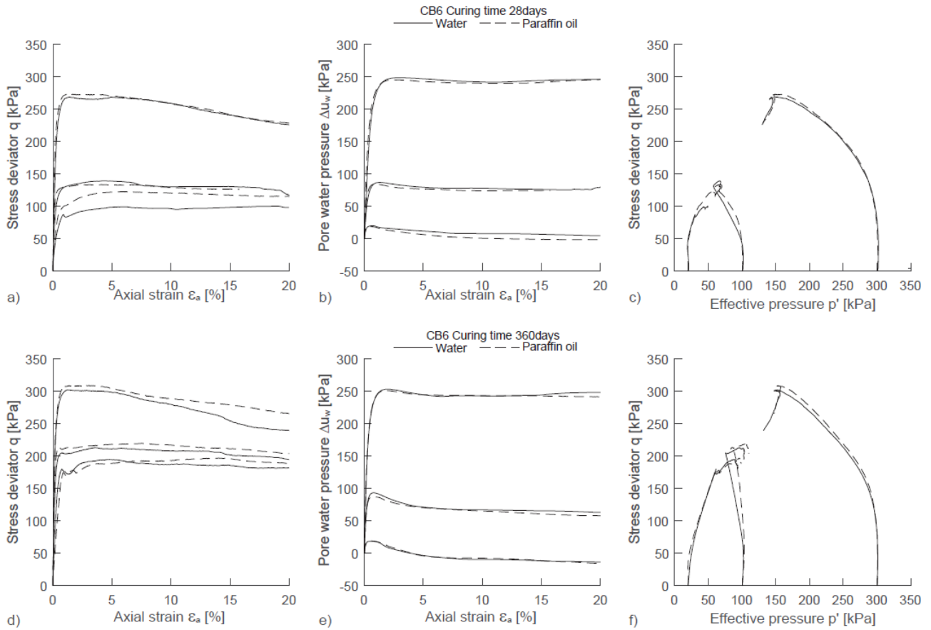
Figure 11: Mixture CB6 triaxial tests ( p'_c=20, 100 and 300 kPa) results: a) q - \epsilon_a plane curing 28 days, b) \Delta u_w - \epsilon_a plane curing 28 days, c) q - p' plane curing 28 days, d) q - \epsilon_a plane curing 360 days, e) \Delta u_w - \epsilon_a plane curing 360 days and f) q - p' plane curing 360 day
