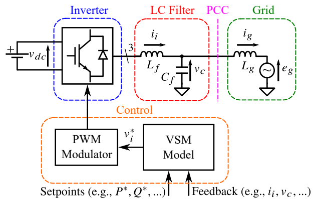
Fig. 1. Considered hardware for VSM implementations.
