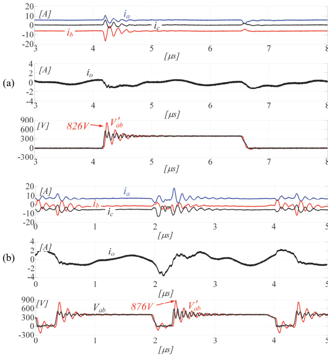
Fig. 7: Example of measured waveforms at 25 kHz and 250 kHz switching frequencies (3 m long cable, 150 ns deadtime, 25 ns risetime).
