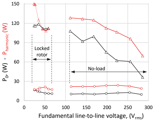
Fig. 23: Common mode losses P_0 and harmonic losses P_{harmonic} vs. the fundamental line-to-line voltage at different switching frequency (circles = 25 kHz, triangles = 200 kHz).
