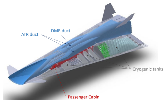
Fig. 1. STRATOFLY MR3 vehicle layout and subsystems integration
