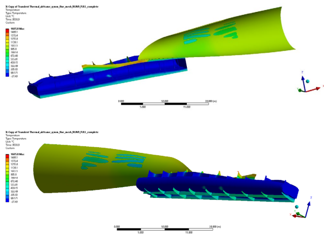
Fig. 28. Temperature map at passenger cabin and surrounding stiffener box structure (a – internal view; b – external view): heat transfer mechanism.
