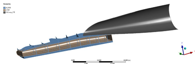
Fig. 29. Passenger cabin, stiffener box, nozzle material distribution.
