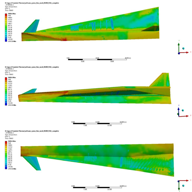
Fig. 25. Temperature map at maximum time instant on external airframe (Mach 8) – a) top view; b) internal view; c) bottom view.
