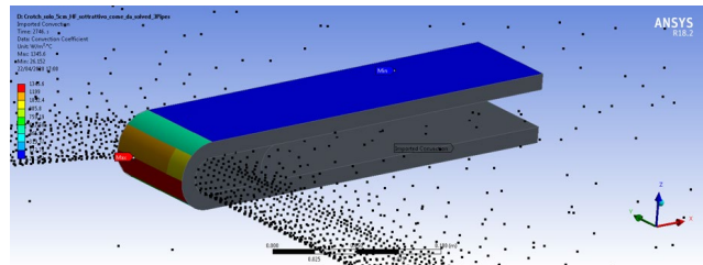
Fig. 14. CFD – structure wet area mis-alignment
