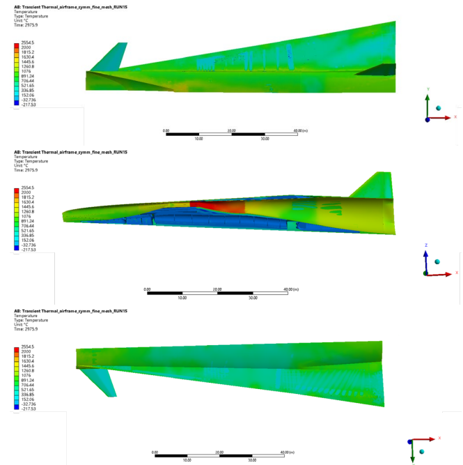
Fig. 24. Temperature map at maximum time instant (Mach 6) – a) top view; b) internal view; c) bottom view.
