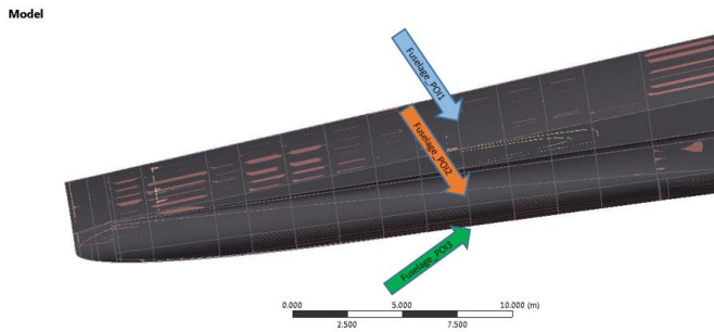
Fig. 9. POI selections on the fuselage
