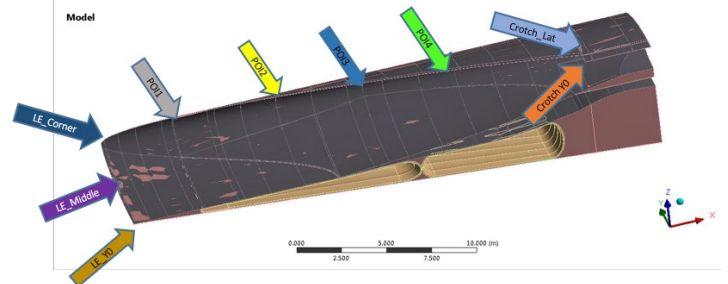
Fig. 7. POI selections on the FEM
