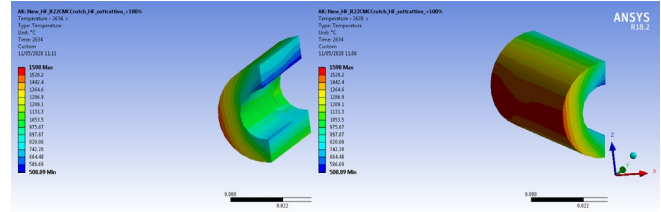
Fig. 18. Thermal map on CMC leading edge at maximum time instant
