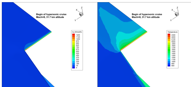
Fig. 5. Flow Temperature and heat transfer coefficient distribution at Mach 8 (crotch area)
