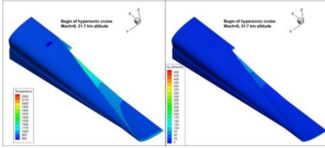
Fig. 3. Flow Temperature and heat transfer coefficient distribution at Mach 8 (ISO view)
