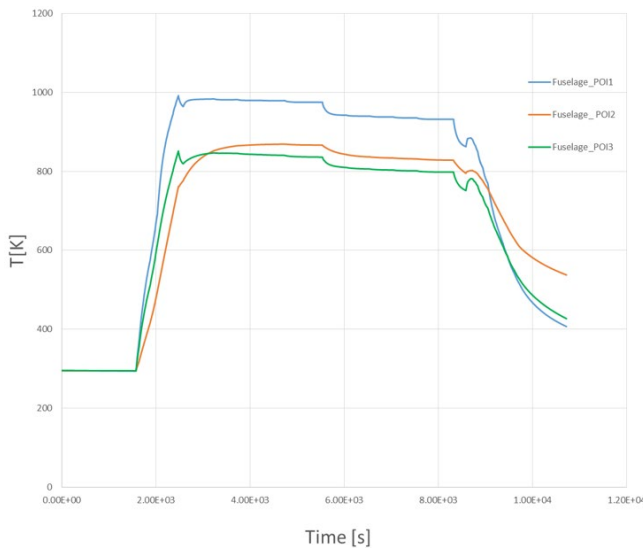
Fig. 10. Fuselage POI thermal behavior
