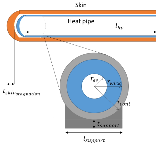
Fig. 12. Most promising heat pipe arrangement
