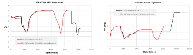
Fig. 2. MR3 Flight Trajectories: Altitude (top left) Mach number (top right), Aerodynamic Efficiency (bottom left) and Angle of Attack (bottom right) time distribution [9]
