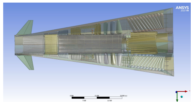
Fig. 18. MR3 geometry layout: different views.
