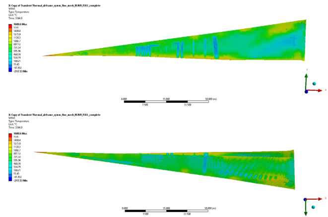
Fig. 26. Temperature map at maximum time instant on the wing (Mach 8) – a) top view; b) bottom view.
