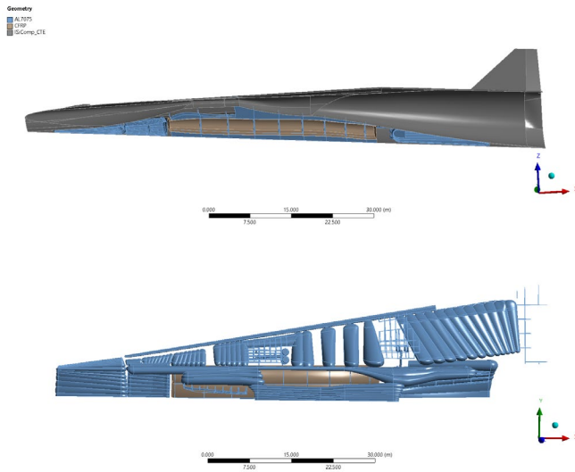
Fig. 19. MR3 Material layout for main structural components, tanks and passenger cabin
