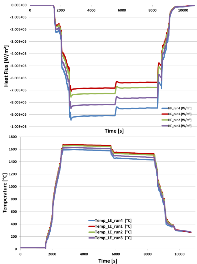
Fig. 17. (a) Subtractive heat fluxes from heat pipe; (b) Maximum temperature evolution at CMC crotch w.r.t different subtractive heat fluxes
