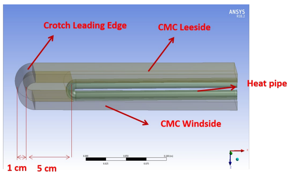
Fig. 13. Crotch geometry basic layout
