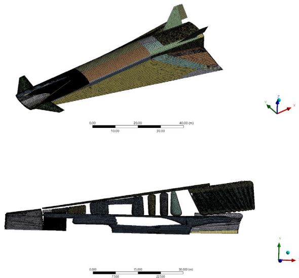
Fig. 20. 3D Mesh for MR3 airframe
