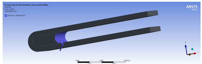
Fig. 15. Subtractive heat flux location
