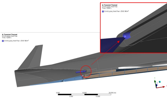
Fig. 22. Subtractive heat flux resulting from the Heat Pipes
