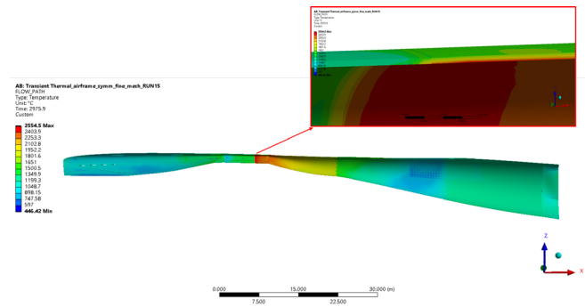
Fig. 30. Temperature map at maximum time instant on the propulsive flow path (Mach 6).
