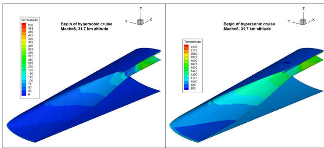
Fig. 4. Flow Temperature and heat transfer coefficient distribution at Mach 8 (internal flow-path view)
