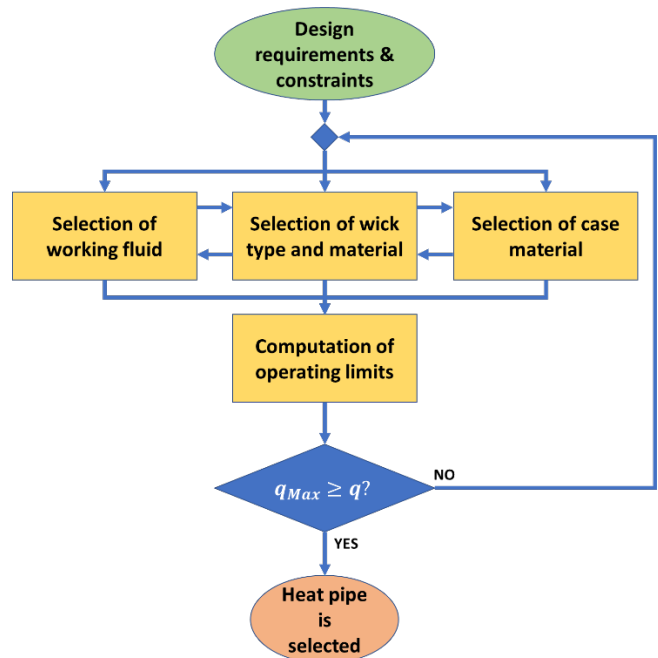
Fig. 11. Heat Pipe sizing process
