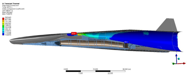
Fig. 23. Imported convection on internal combustion chamber surfaces.
