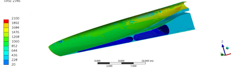
Fig. 6. Thermal map at Mach 8
