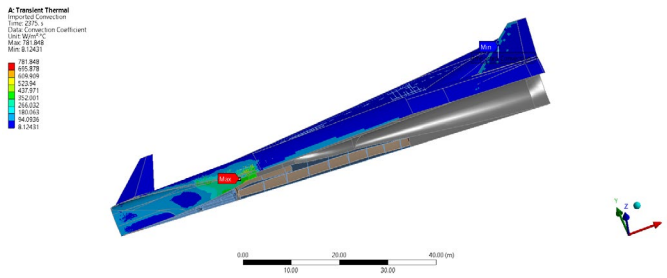
Fig. 21. Imported convection on external surfaces
