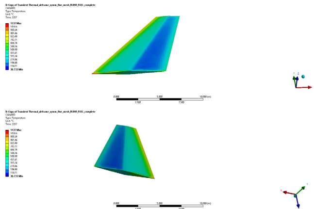
Fig. 27. Temperature map at maximum time instant on the canard (Mach 8) – a) leeside view; b) windside view.
