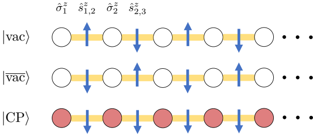
Figure 1: (Color online). Product states relevant to the quenches in the U(1) quantum link model (1), the dynamics of which we numerically calculate using Krylov subspace methods. The vacua |\text{vac}\rangle and |\overline{\text{vac}}\rangle are the doubly degenerate ground states of Eq. (1) at \mu \rightarrow \infty in the physical sector \hat{G}_j |\phi\rangle = 0, \forall j . They both break the global \mathbb{Z}_2 symmetry of this model. They lead to resonant scarring when they are quenched with Eq. (1) at \mu = 0 . The charge-proliferated or “polarized” state |\text{CP}\rangle is the nondegenerate \mathbb{Z}_2 -symmetric ground state of Eq. (1) at \mu \rightarrow -\infty in the physical sector \hat{G}_j |\phi\rangle = 0, \forall j . It leads to detuned scarring when quenched by Hamiltonian (1) with a finite mass around \mu = -0.84J . Unless otherwise stated, we employ in our numerics a system size of L_m = L = 12 lattice sites and L_g = L - 1 = 11 gauge links with open boundary conditions.
